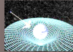
Space-time
